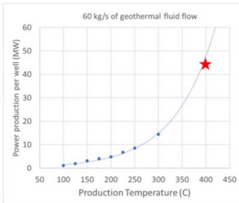
Figure 7-22. Geothermal power production compared to production temperature.
